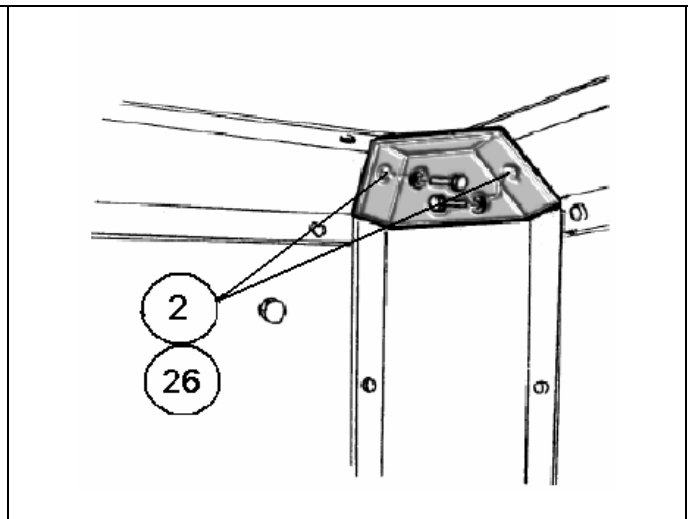
Figure 5-40. Roof Kit Installation - Right rear Corner (8 of 10).
