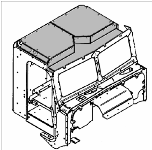
Figure 5-31. Roof Kit Installation – Final View.
