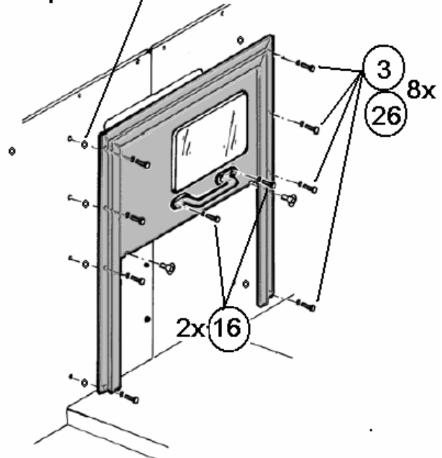
Figure 5-58a. Emergency Exit Kit Installation (2 of 4).
