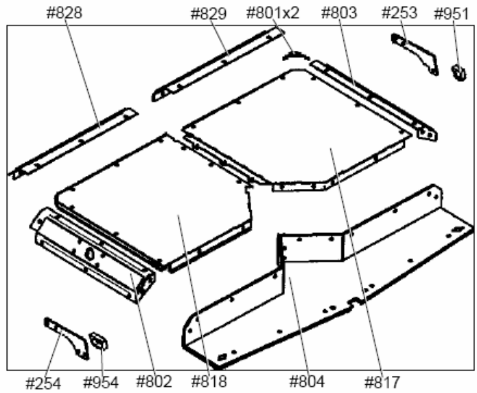
Figure 5-32. Roof Kit Installation – Parts.
