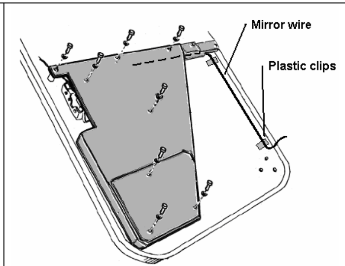
Figure 5-115. LH Door Accessories Assembly - Reassembly of Armored Door (6 of 6).
